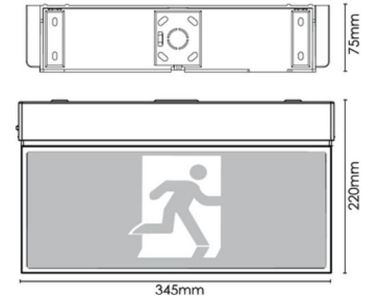
EXS-EDGE (Surface Mounted):
